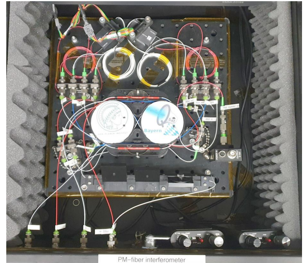
Interferometer 1 and 2 integrated setup [B. Hacker et al 2023 New J. Phys. 25 113007]
